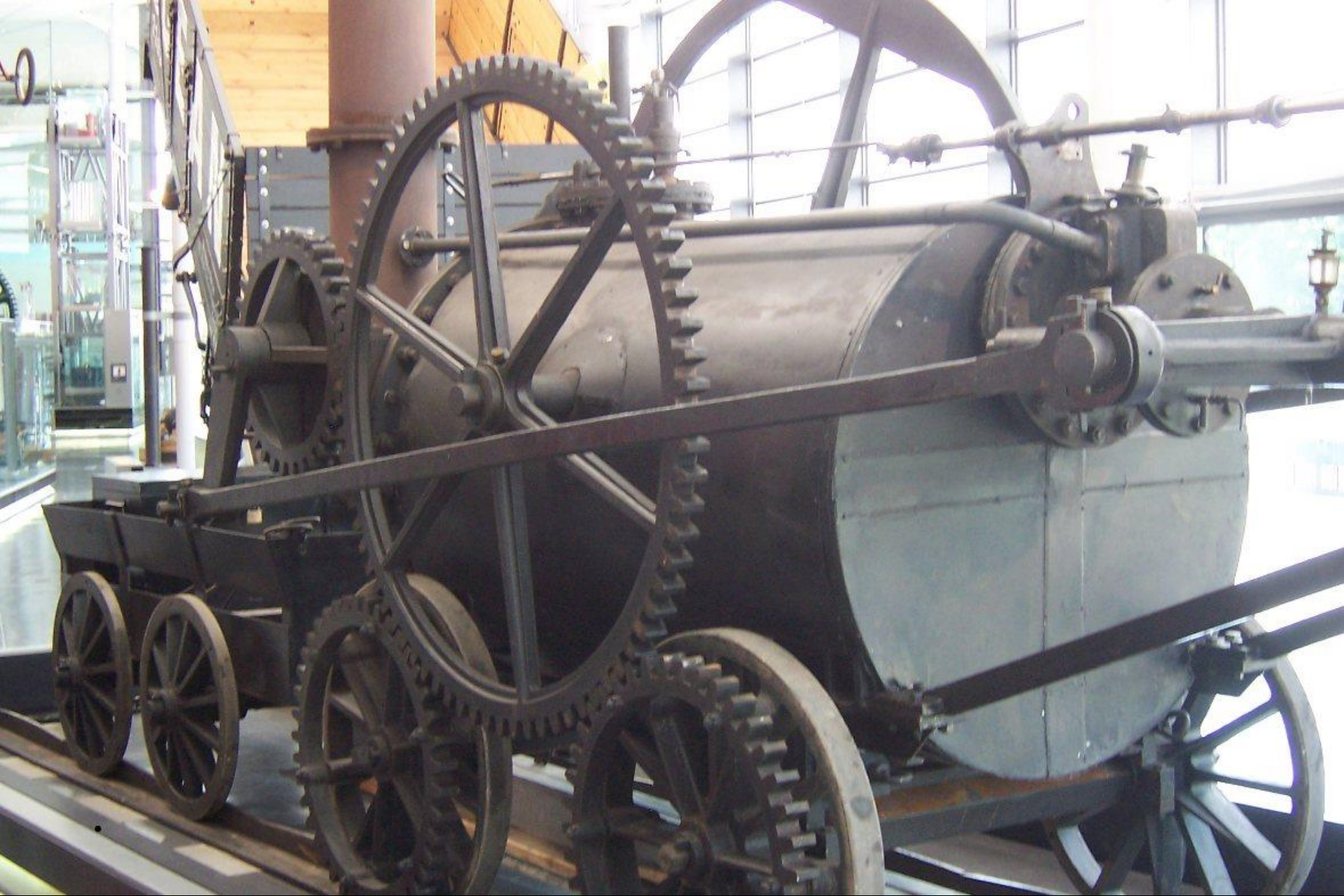
Replica of Trevithick's 1804 locomotive, Creative Commons License
